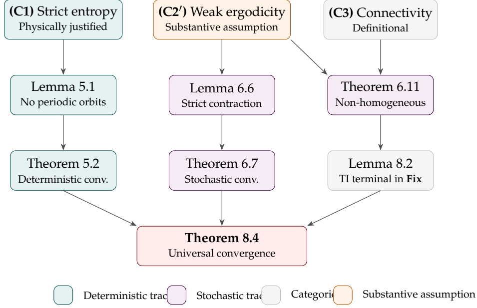
Figure 1: Proof dependency diagram. The three conditions (top row) feed into intermediate lemmas (middle) and the main theorems (bottom), culminating in Theorem 8.4. Colour encodes the proof track: teal for deterministic, purple for stochastic, grey for categorical, and amber for the single substantive physical assumption (C2').
